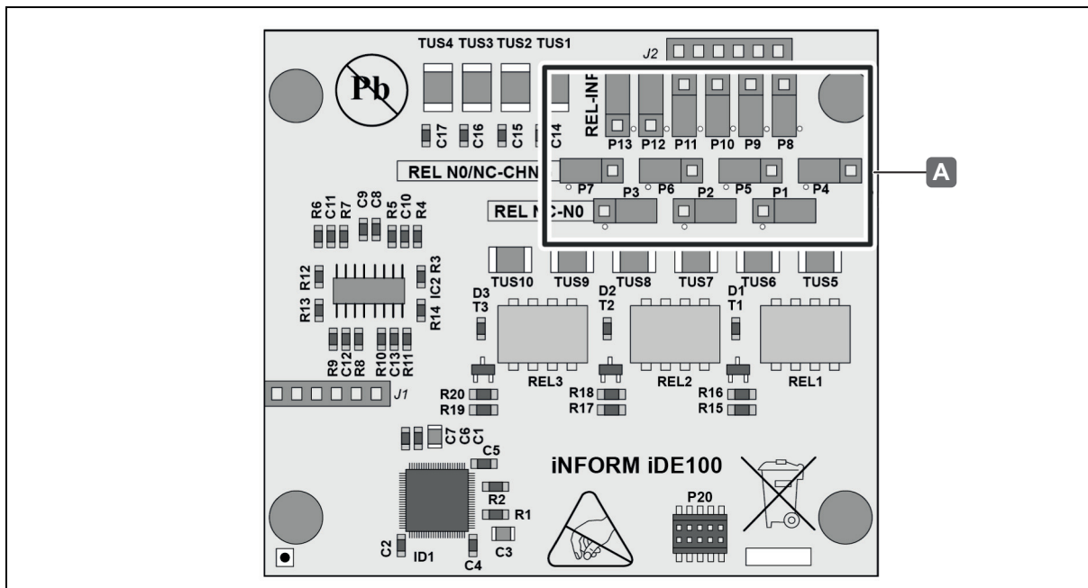
Fig. 19: WTX 200 - position of the jumpers when used for 2 additional relay output ports and 1 additional analogue/digital input port
