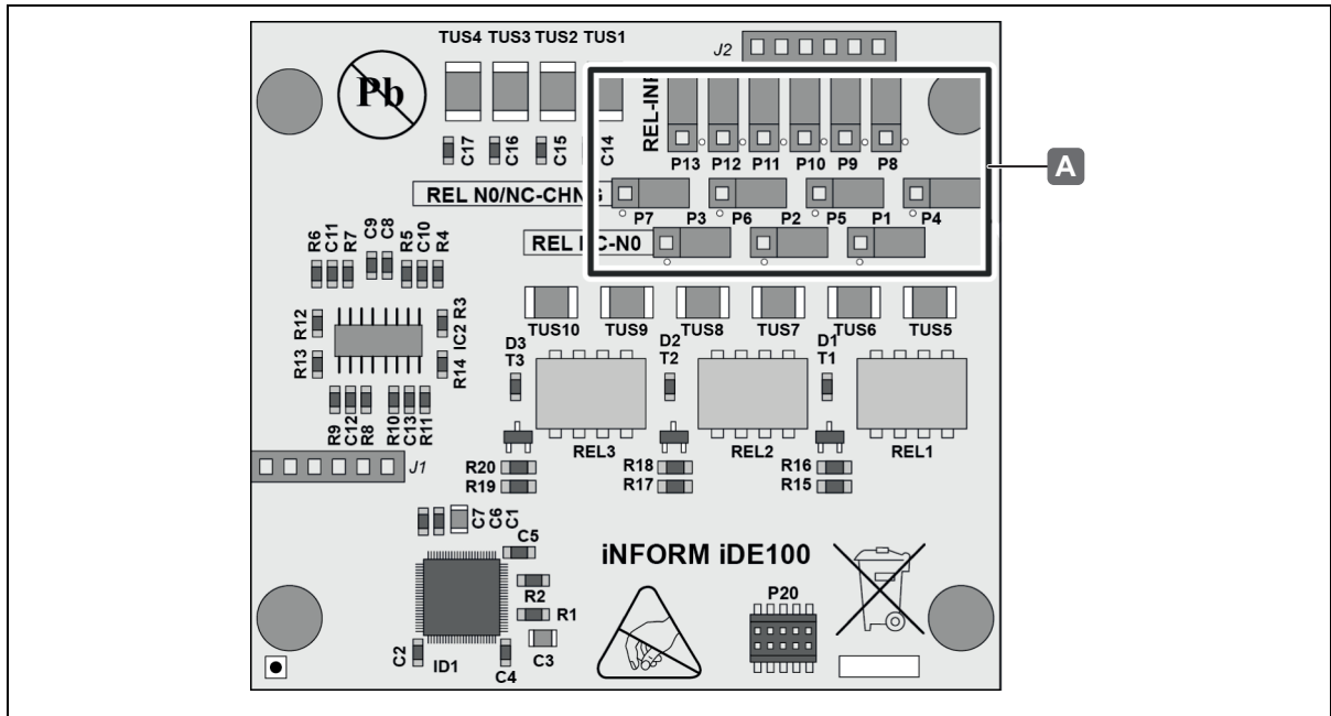
Fig. 18: WTX 200 - position of the jumpers when used for additional analogue/digital input ports
