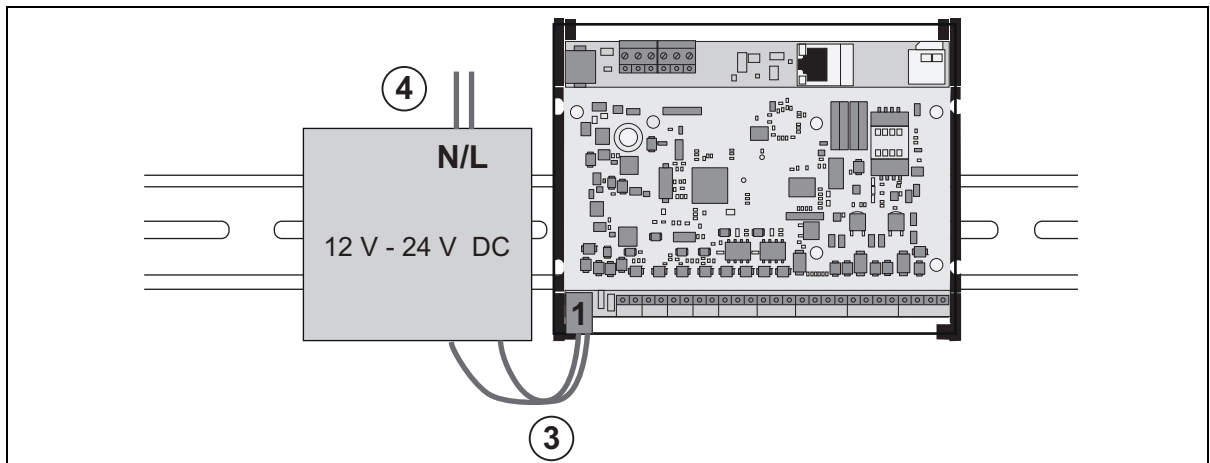
Abb. 6: Montage WTC 200
