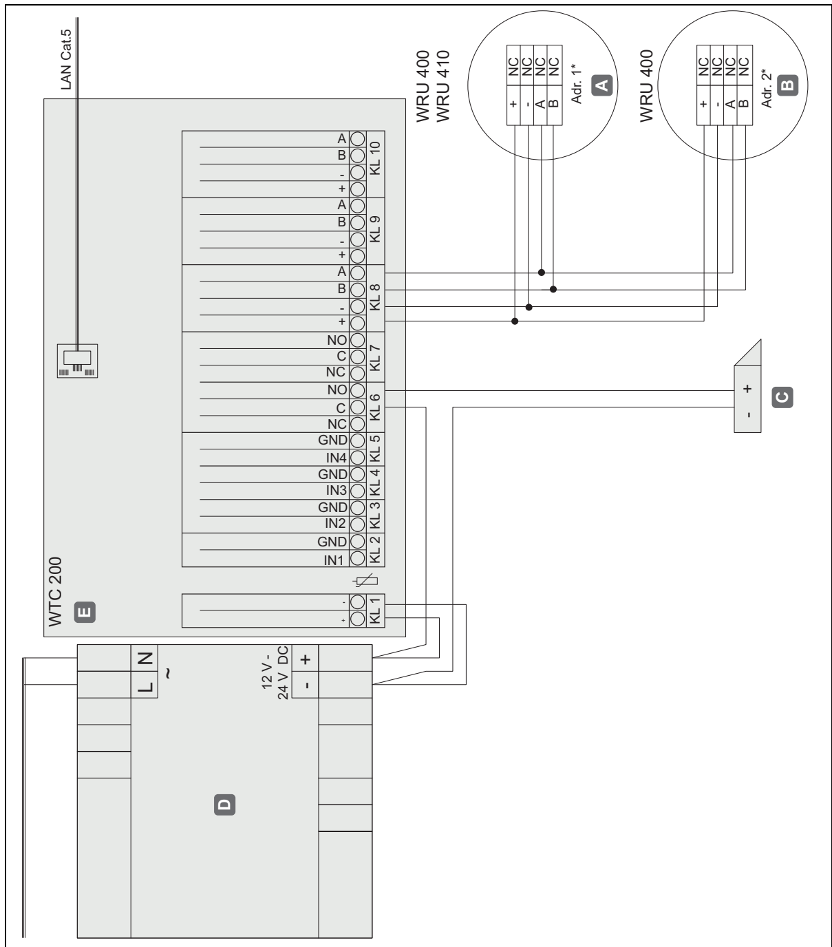
Fig. 28: Circuit diagram for installation example 3
