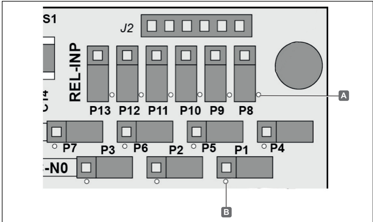
Fig. 17: WTX 200 connections - position connection no. 1 (white dot)
