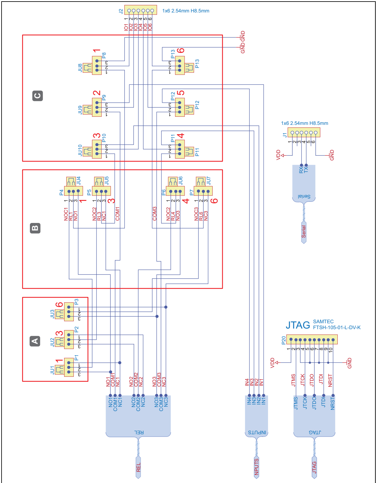
Fig. 16: Structure and pin assignment of the WTX 200
