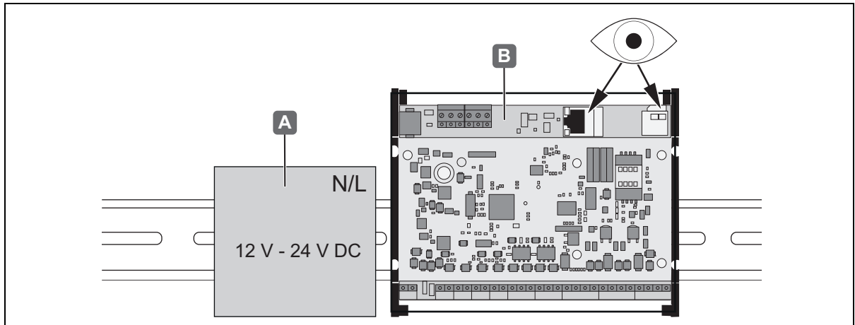
Abb. 5: Montage WTC 200
