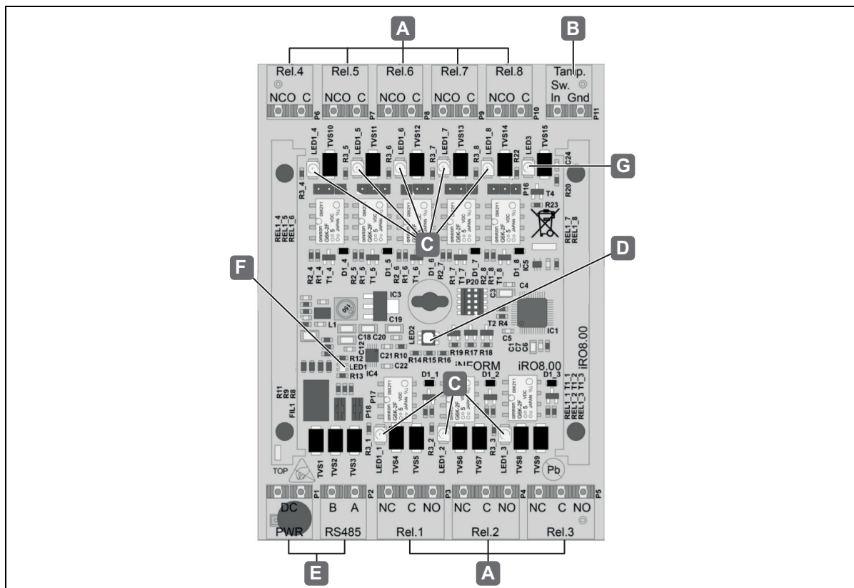
Fig. 20: WTX 201 connections
