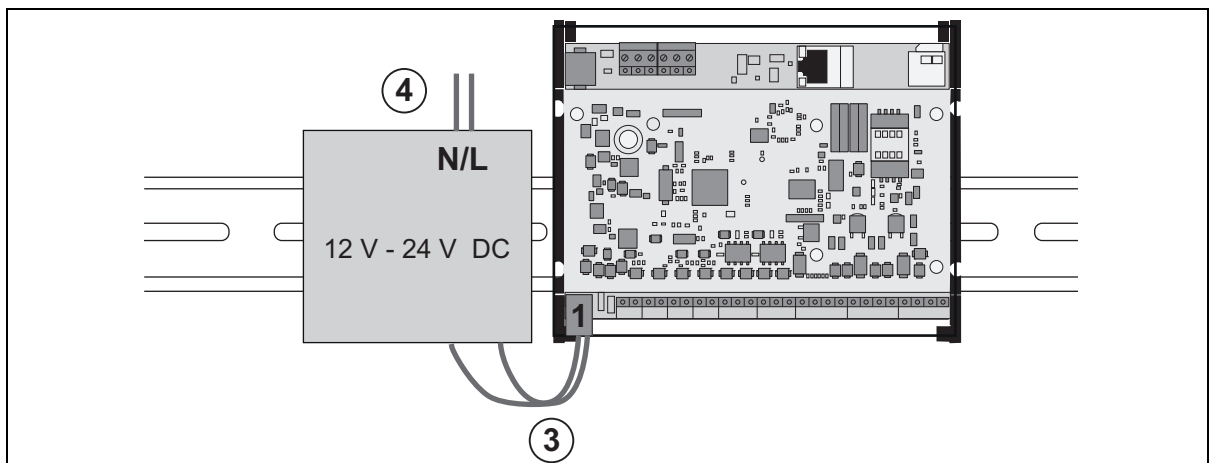
Fig. 6: WTC 200 installation
