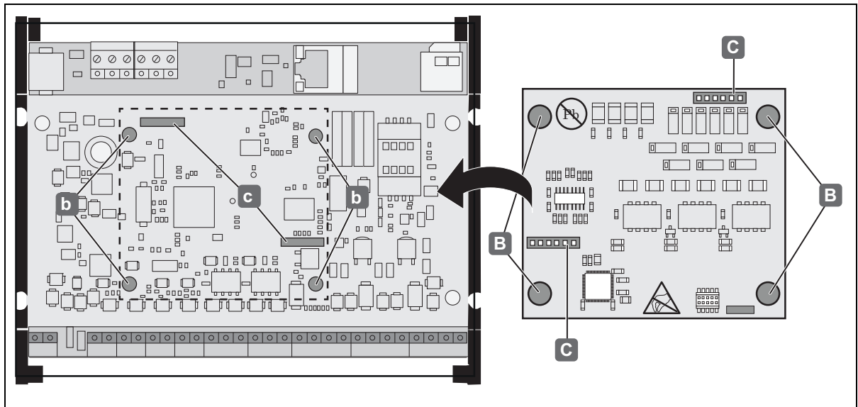
Fig. 9: WTX 200 Installation - clipping WTX 200 onto WTC 200 controller
