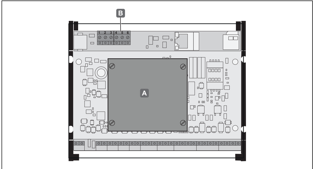
Fig. 15: WTX 200 connections
