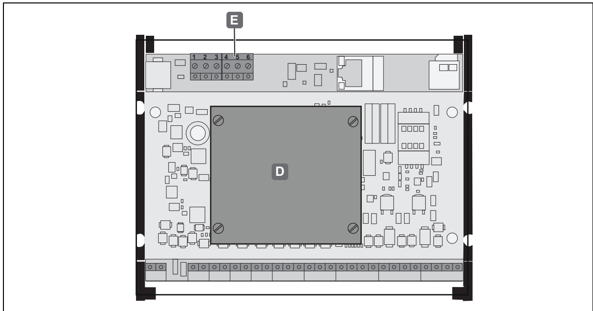
Fig. 10: WTX 200 installation - connected to controller
