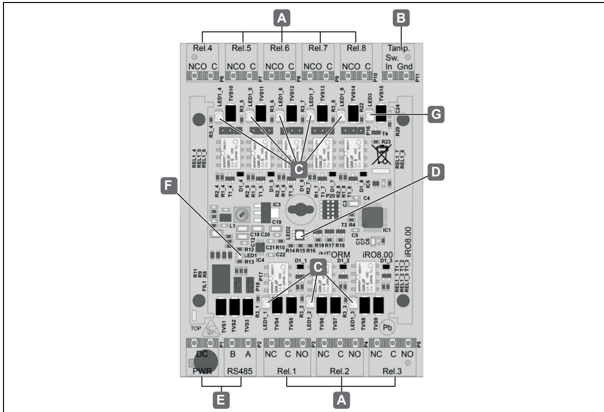
Abb. 20: Anschlüsse WTX 201
